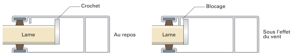
Figure 136 : Crochet anticyclonique
