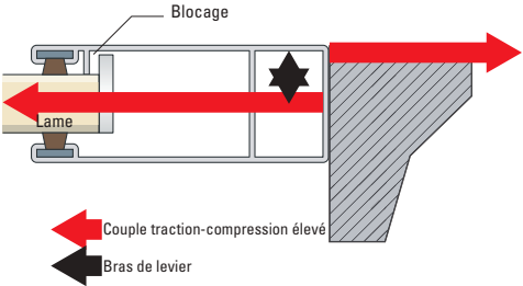
Figure 138 : Coulisse standard Disposition vulnérable
